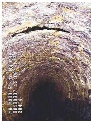
Holes in pipe wall at 246' & 284'
